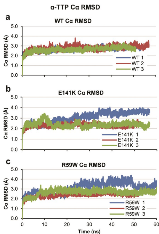
Figure 2. \alpha rmsd values over time for all three proteins. Values were calculated using \alpha -carbons excluding both termini and \alpha 14 . (a) Wild type. (b) E141K. (c) R59W.
