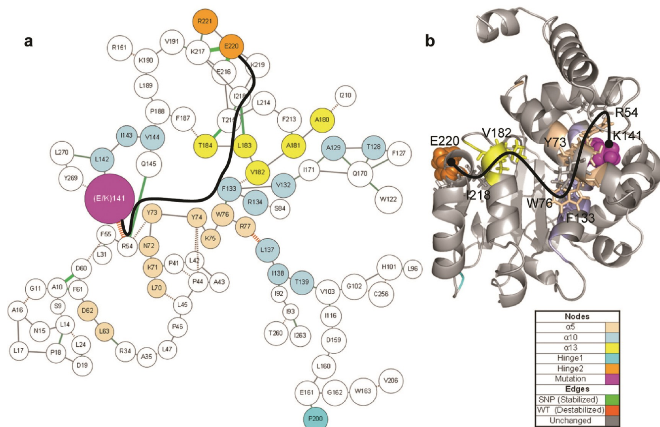
Figure 7. Contact disruption pathways in the E141K mutant. Contact occupancy differences were calculated between all wild-type simulations and all E141K simulations with a significance threshold of 0.09, an allowable traversal threshold of 0.06, and a search depth of 2. (a) ContactWalker disruption pathways. The thickness of the line indicates the magnitude of the occupancy change; green lines indicate mutant-associated stabilization, and orange lines indicate mutant-associated destabilization. Nodes are colored per the legend. The black line highlights a pathway between the mutation site and the hinge 2 region. (b) The 51 ns structure of E141K simulation 1. The black line indicates the same pathway that is labeled in panel a. Pathway residues are rendered as sticks and labeled for orientation. The K141 mutation site is rendered as magenta spheres. The final residue of the pathway (E220) is rendered as orange spheres.
