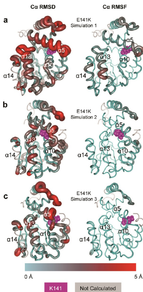
Figure 6. Representative E141K structures rendered as tubes. The tube radius and color reflect the Ca rmsd (left) and Ca rmsf (right). The K141 mutation site is rendered as magenta spheres. Simulations 1 (a), 2 (b), and 3 (c).
