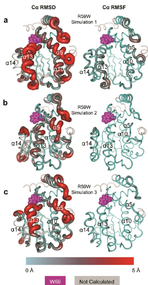
Figure 8. Representative R59W structures rendered as tubes. The tube radius and color reflect \text{Ca} rmsd (left) and \text{Ca} rmsf (right). The W59 mutation site is rendered as magenta spheres. Simulations 1 (a), 2 (b), and 3 (c).
