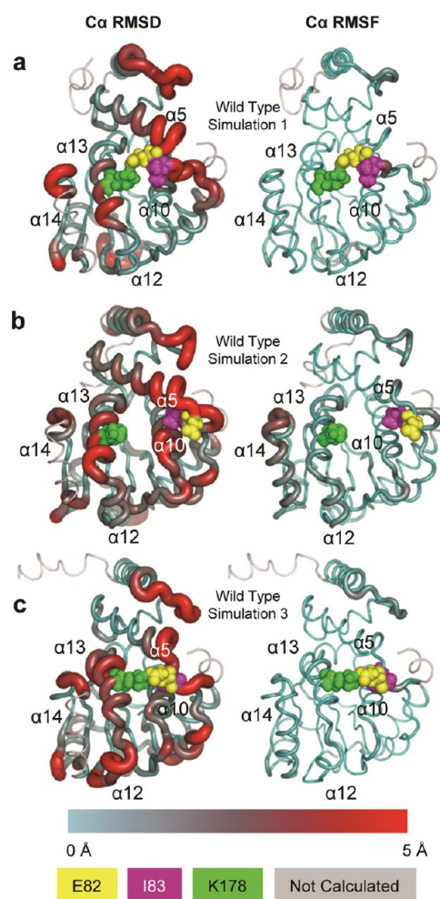
Figure 5. Representative wild-type structures rendered as tubes. The tube radius and color reflect the \alpha rmsd (left) and \alpha rmsf (right). E82, I83, and K178 are colored per the legend and rendered as spheres. Simulations 1 (a), 2 (b), and 3 (c). Note the separation of K178 from E82 and I83 in simulation 2.
