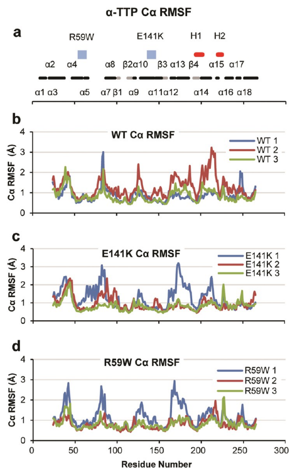
Figure 3. \alpha rmsf calculated using \alpha -carbons and excluding both termini. (a) Black and gray bands indicate \alpha -helices and \beta -sheets, respectively; blue squares indicate mutation sites, and red bands indicate hinge regions 1 and 2 (labeled H1 and H2, respectively). (b) Wild type. (c) E141K mutant. (d) R59W mutant.
