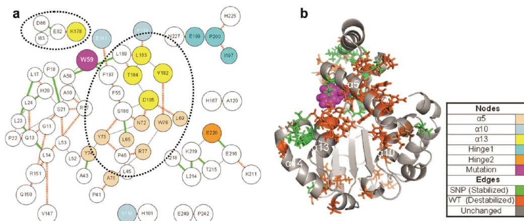
Figure 9. Contact disruption pathways in the R59W mutant. The contact occupancy difference was calculated between simulation 2 and simulations 1 and 3 with a significance threshold of 0.9, an allowable traversal threshold of 0.9, and a search depth of 1. (a) ContactWalker disruption pathways. The thickness of the line indicates the magnitude of the occupancy change; green lines indicate stabilization of the mutant, and orange lines indicate mutant destabilization. Nodes are colored per the legend. The dotted circles highlight destabilized \alpha 13 residues. (b) The 51 ns structure of R59W simulation 1. Significant nodes are rendered as sticks and colored on the basis of the overall stability (green) or instability (orange). Note the prevalence of destabilized residues among \alpha 5 , \alpha 10 , and \alpha 13 coincident with the expansion of the ligand binding pocket.
