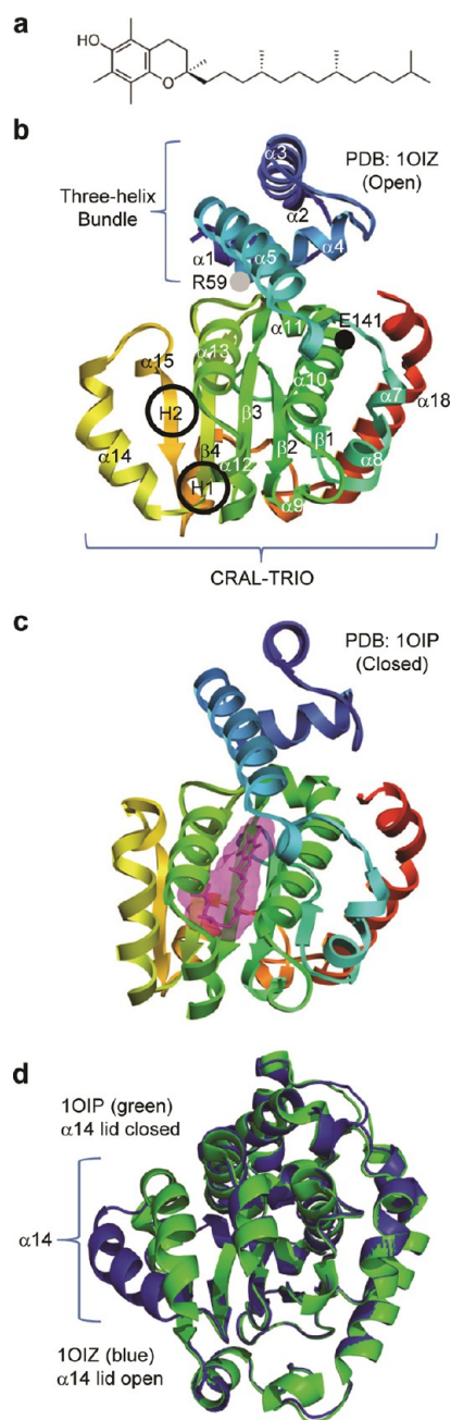
Figure 1. Molecular structures of vitamin E and the different forms of \alpha -TTP. (a) RRR- \alpha -tocopherol (vitamin E). (b) In the unbound structure (PDB entry 1OIZ), a lid formed by the \alpha 14 region is open, allowing entrance to a hydrophobic binding pocket. The CRAL-TRIO domain is indicated in brackets. The black and gray filled circles indicate the E141K and R59W mutation regions, respectively. The two hinge regions are circled and labeled as H1 and H2. (c) In the bound conformation (PDB entry 1OIP), the lid is closed, enclosing the binding pocket. (d) 1OIZ (blue) and 1OIP (green) overlaid and aligned by C \alpha rmsd. The C \alpha rmsd between the two structures excluding \alpha 14 was 0.5 Å.
